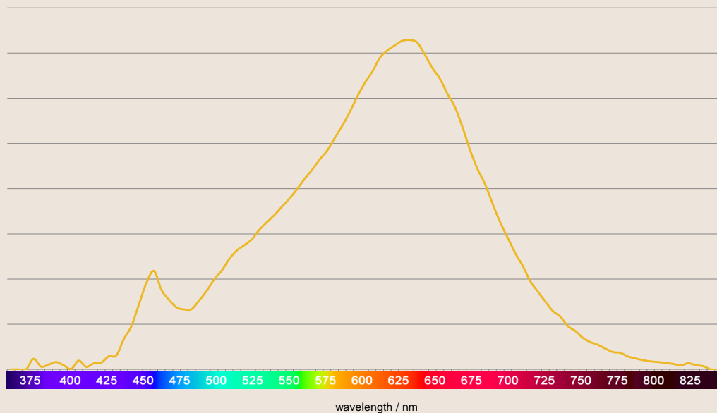
SPECTRAL POWER DISTRIBUTION OF LEDON 6W MR16 GU10
